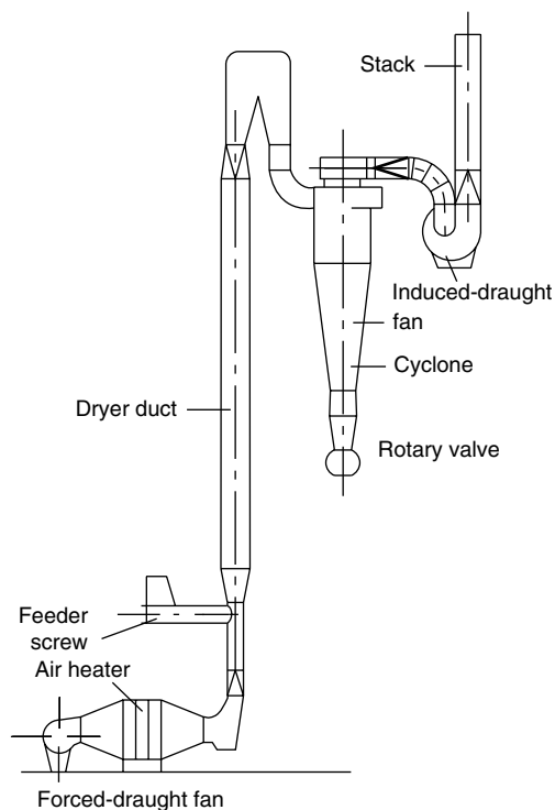
Figure 10.29. Pneumatic dryer
