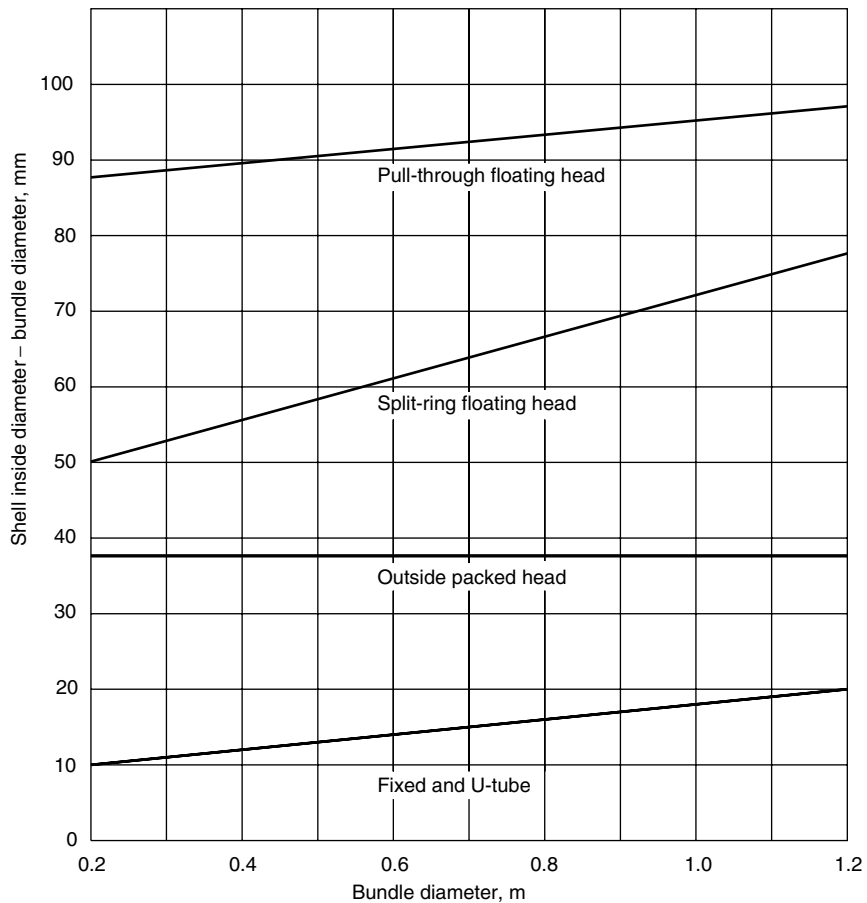
Figure 12.10. Shell-bundle clearance
