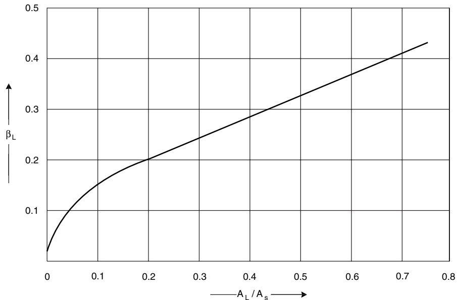
Figure 12.35. Coefficient for F_L , heat transfer
