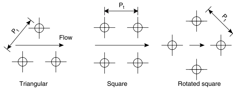
Figure 12.9. Tube patterns
