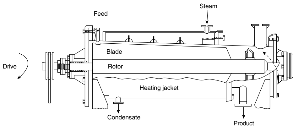
Figure 10.34. Horizontal wiped-film evaporator
