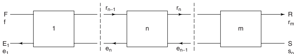
Figure 11.57. Counter-current extraction
