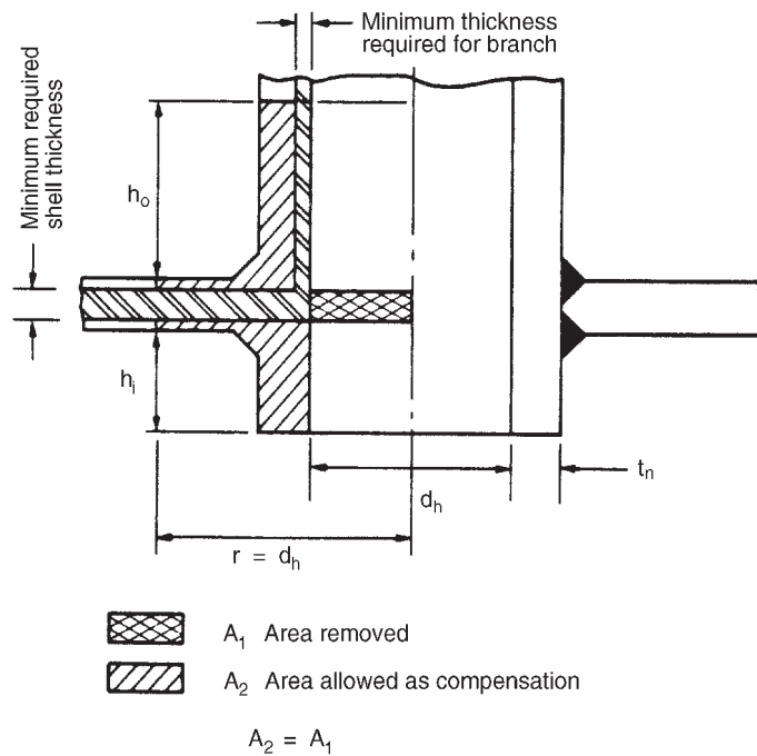
Figure 13.13. Equal-area method of compensation
