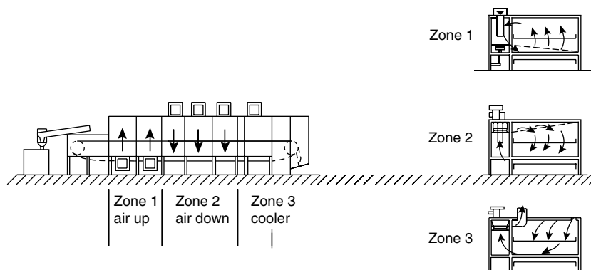
Figure 10.26. Conveyor dryer
