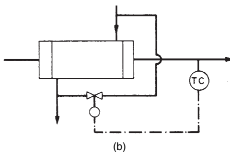
Figure 5.19. (a) Control of one fluid stream (b) By-pass control
