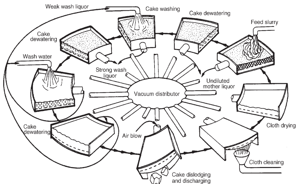
Figure 10.15. Pan filters
