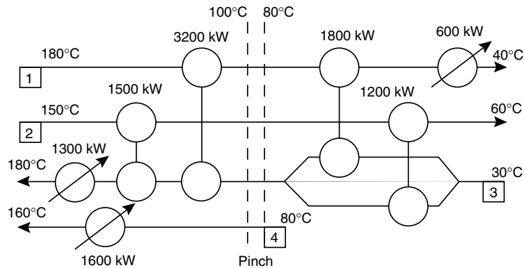
Figure 3.31. Network, example 3.17
