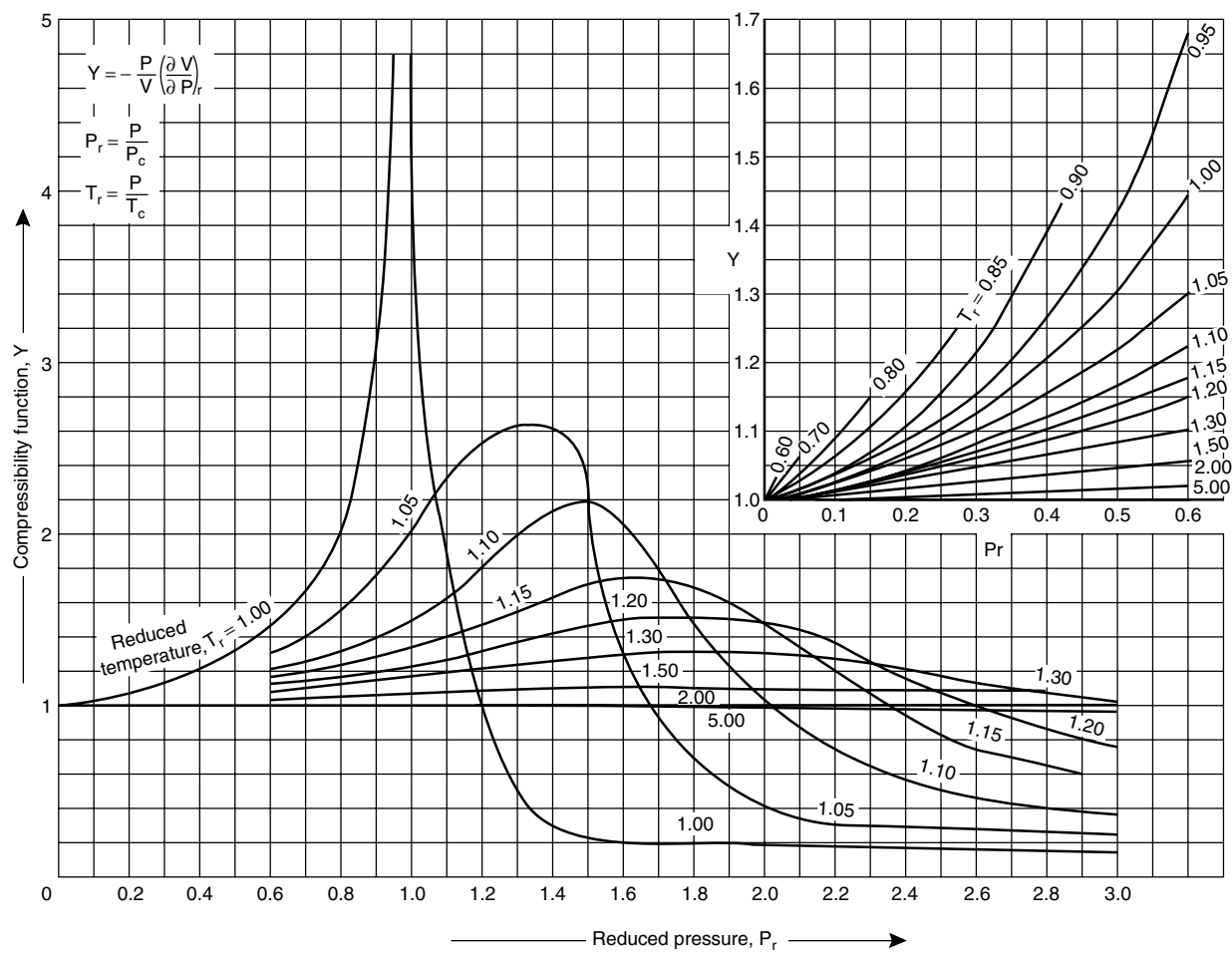
Figure 3.10. Generalised compressibility function Y
