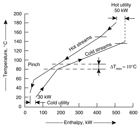
Figure 3.22. Hot and cold stream composite curves
