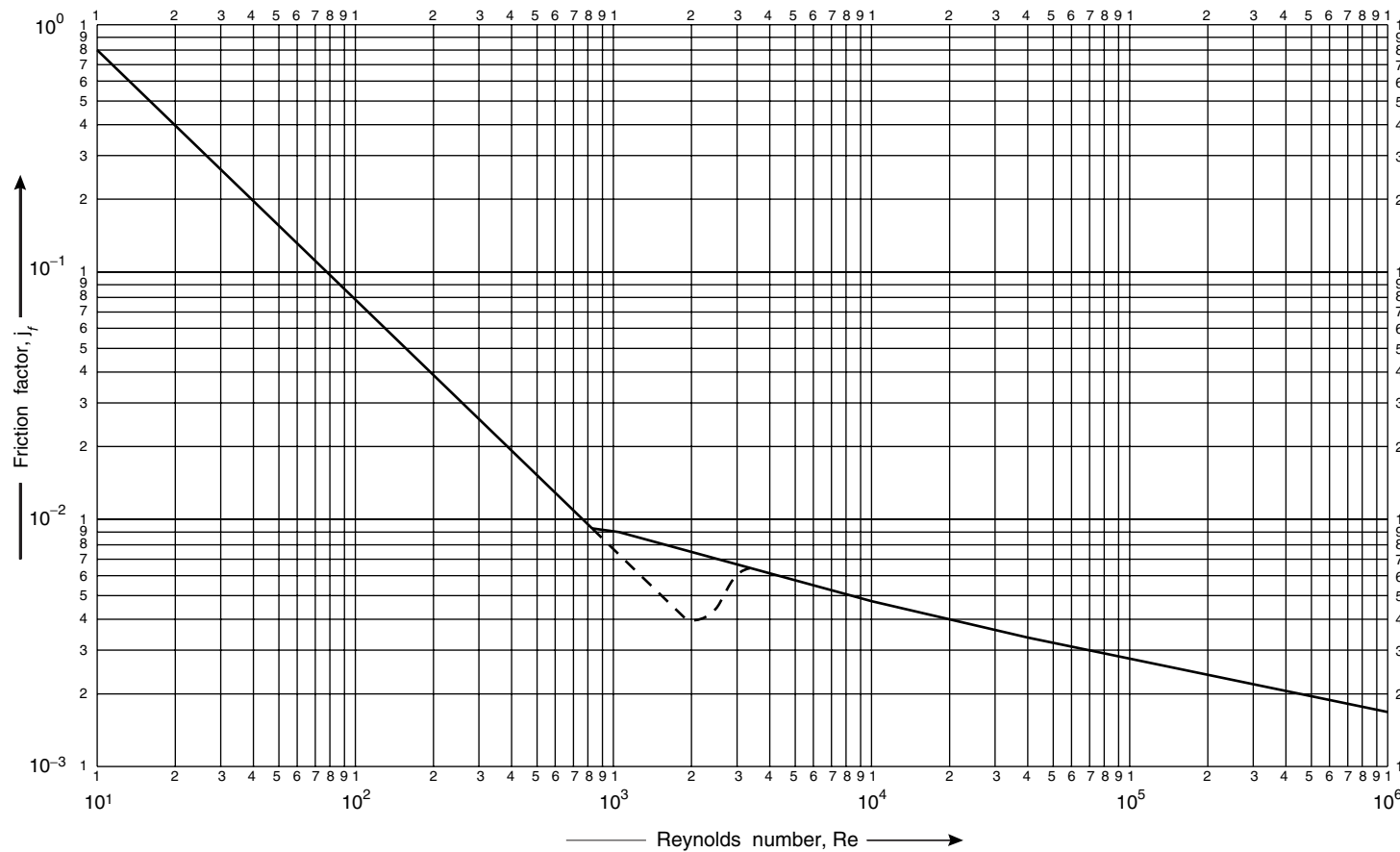
Figure 12.24. Tube-side friction factors
