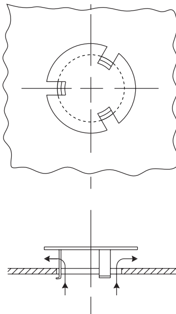
Figure 11.20. Simple valve
