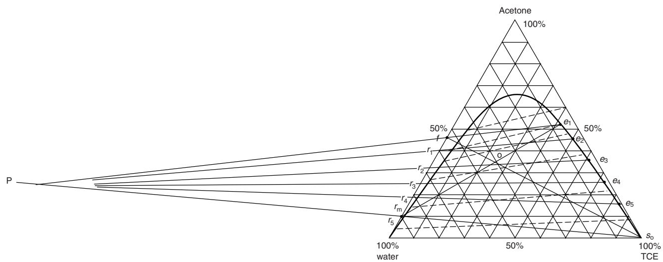
Figure 11.58. Example 11.15
