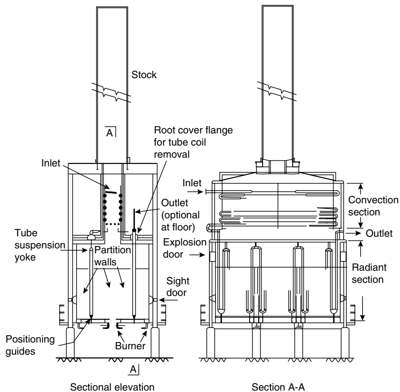
Figure 12.70. (Foster Wheeler) Multi-zoned pyrolysis furnace
