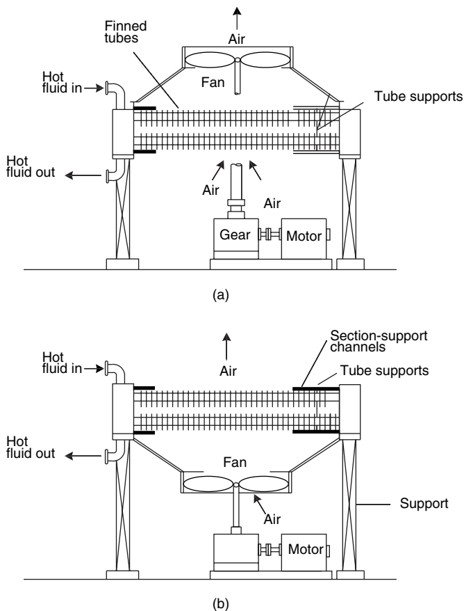
Figure 12.68. Air-cooled exchangers
