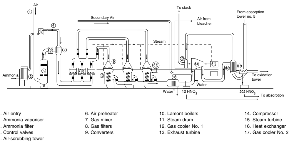
Figure 3.14. Connections of a nitric acid plant, intermediate pressure type
