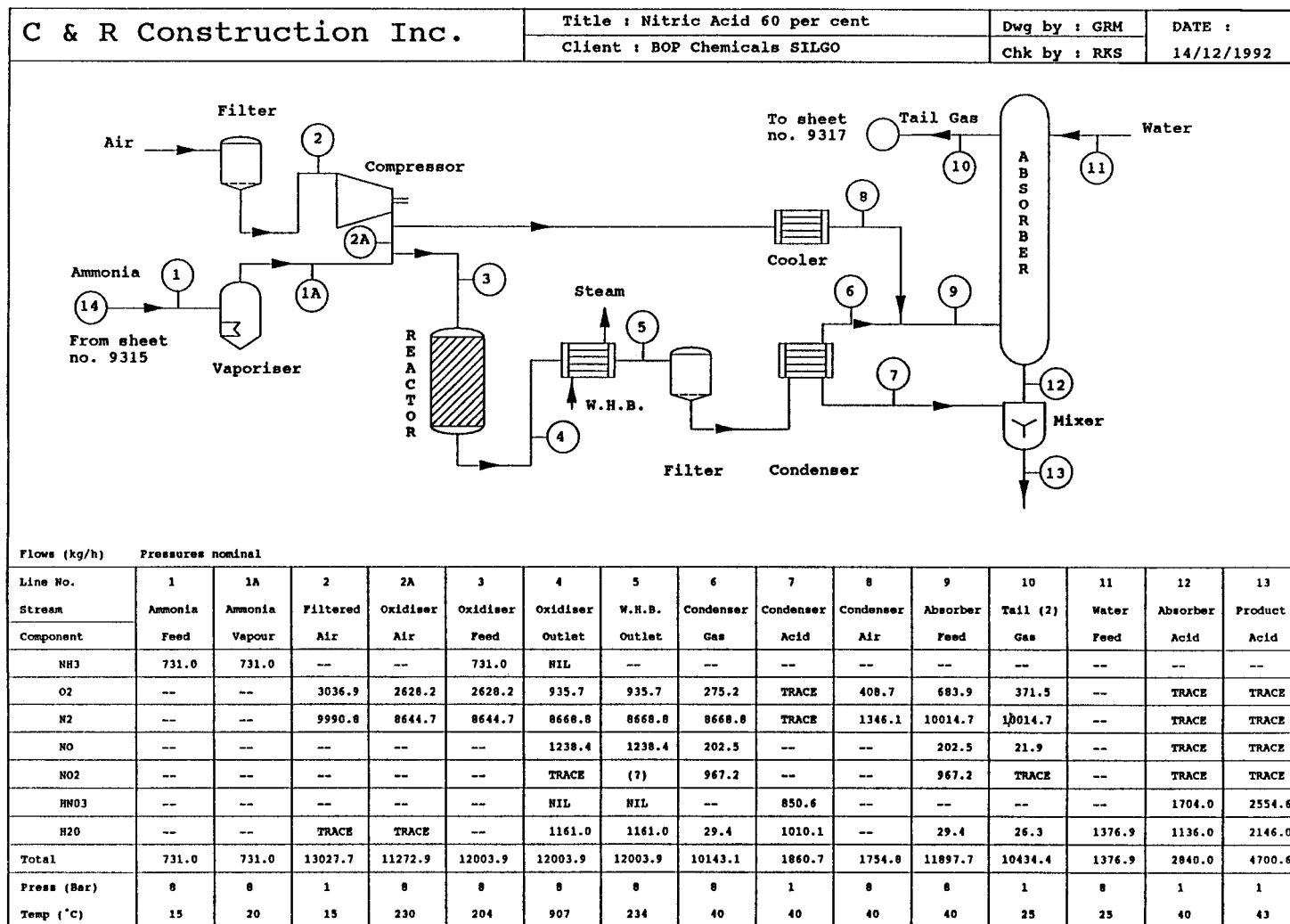
Figure 4.2a. Flow-sheet drawn using FLOSHEET
