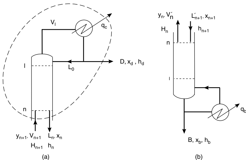
Figure 11.4. Column flows and compositions (a) Above feed (b) Below feed
