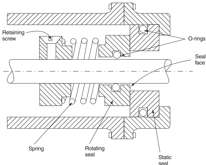
Figure 5.14. Basic mechanical seal
