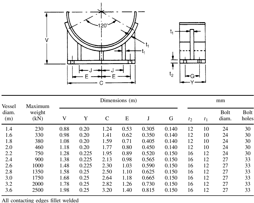
Figure 13.26. (b) for vessels greater than 1.2 m
