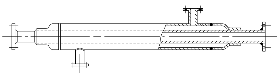
Figure 12.67. Double-pipe exchanger (constructed for weld fittings)
