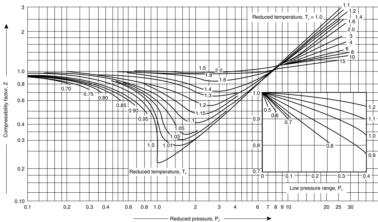
Figure 3.8. Compressibility factors of gases and vapours
