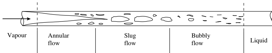
Figure 12.44. Flow patterns, vapour condensing in a horizontal tube
