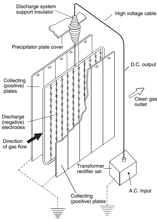
Figure 10.50. Electrostatic precipitator
