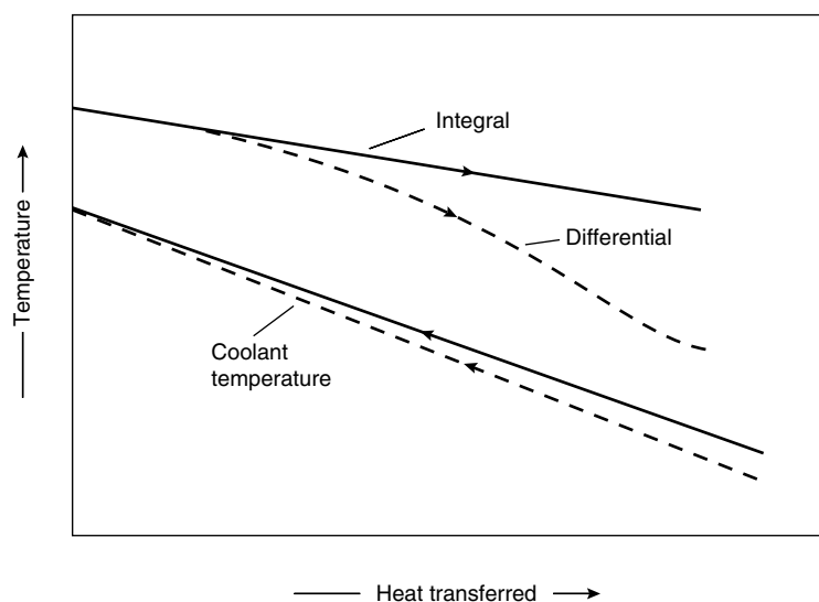
Figure 12.48. Condensation curves
