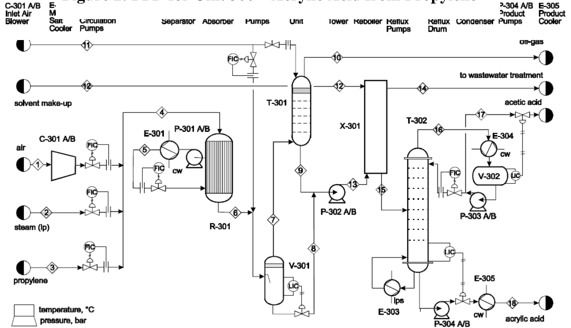
Figure 2: PFD for Unit 300 – Acrylic Acid from Propylene
